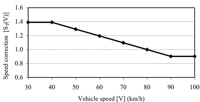
Figure 3-2 Speed correction factor for tyre wear particle emissions
